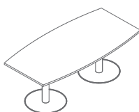
ST12P 2000 / 800-1000 / 730 96.5 kg
